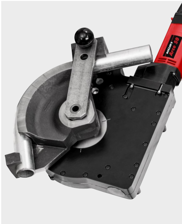
Square driver 10-40, Support 10-40
