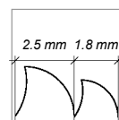
Combi-teeth
